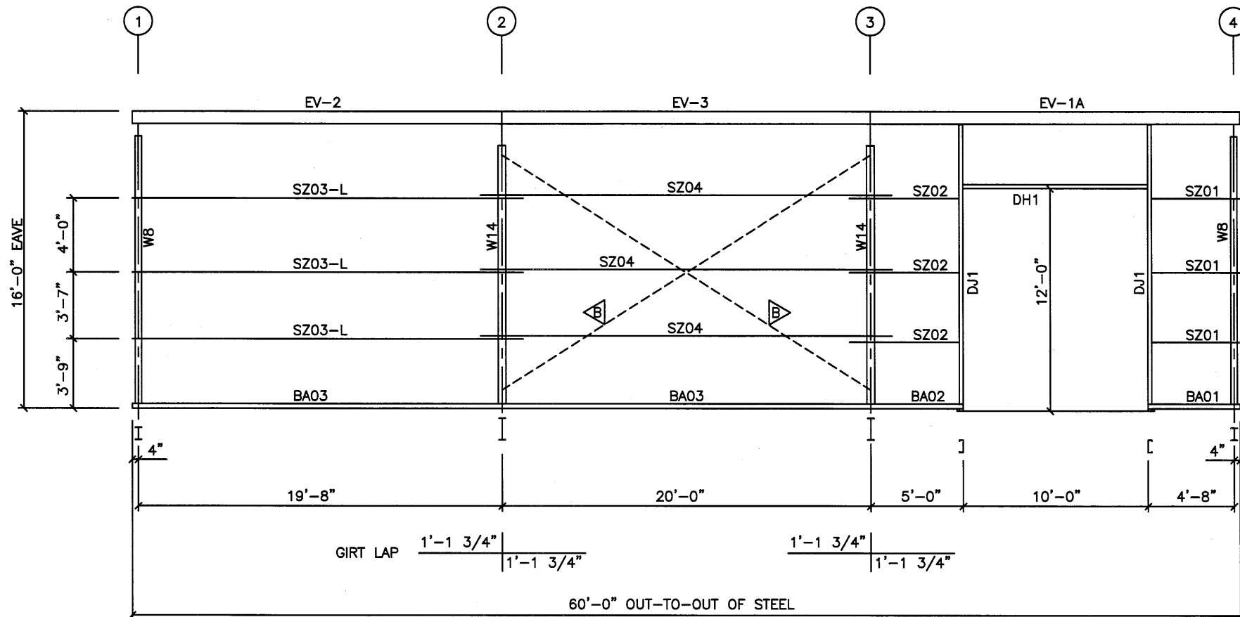
SIDEWALL FRAMING ELEV. @ COL. LINE A N.T.S.
