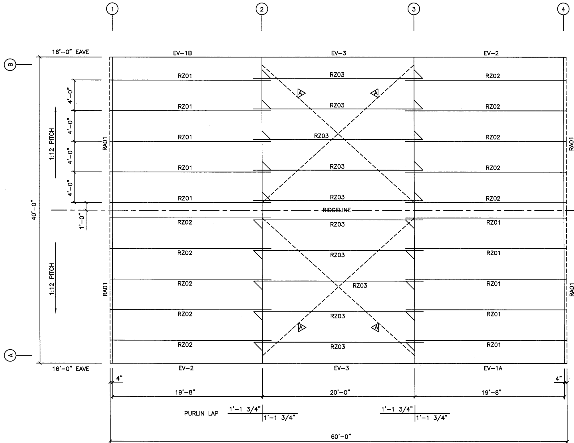
ROOF FRAMING PLAN N.T.S.
