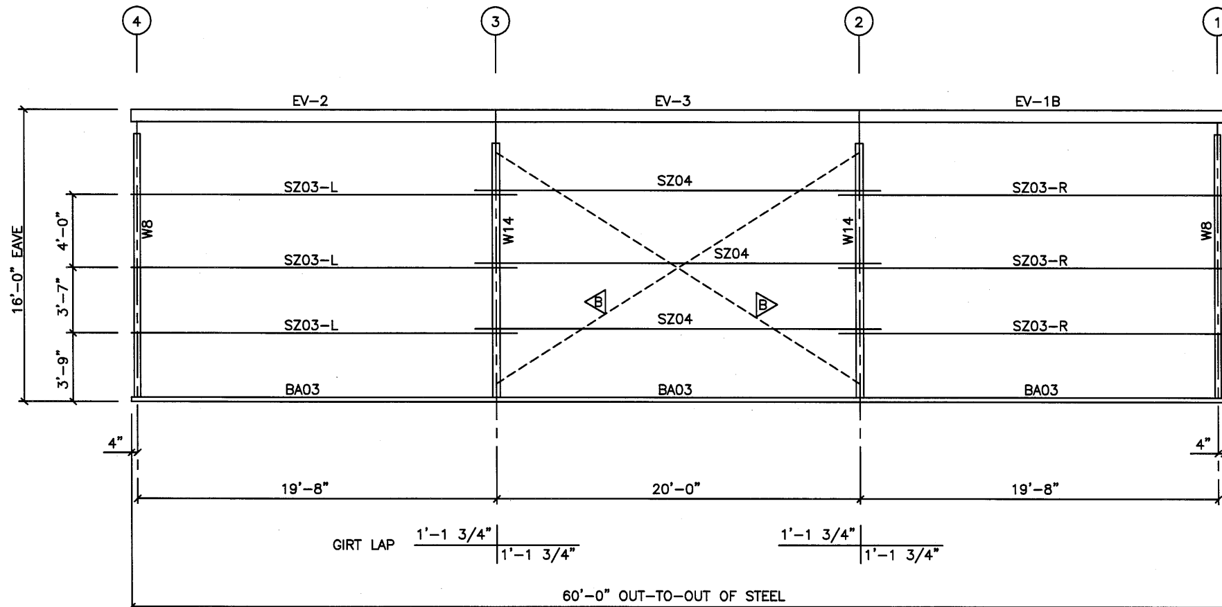
SIDEWALL FRAMING ELEV. @ COL. LINE B N.T.S.
